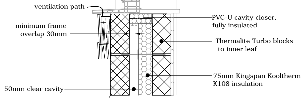
Typical Section
